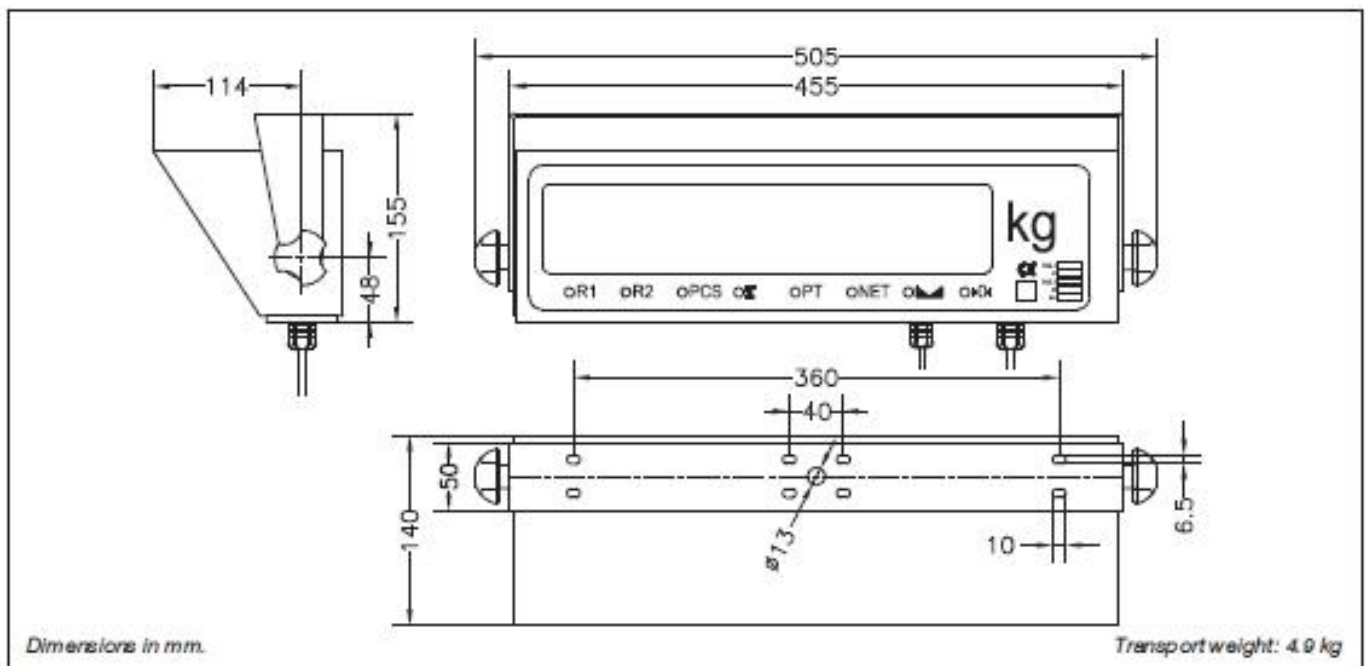
89316 Remote Display RD 60
