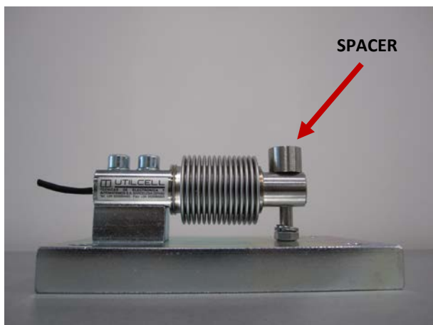
Spacer mounting
